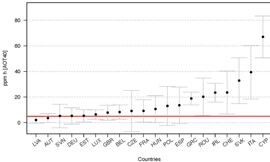
Figure 5-3. Mean AOT40 for 20 countries based on April–September passive ozone concentration values from 2000–2013.
