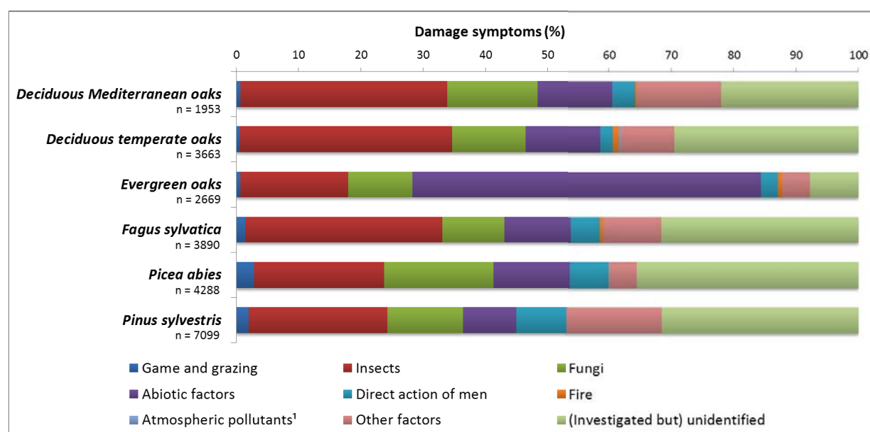
Figure 3-31. Damage symptoms according to agent group in the main tree species and species groups on Level I plots. 1 Visible symptoms of direct atmospheric pollution impact only (cf. Figure 3-1).
