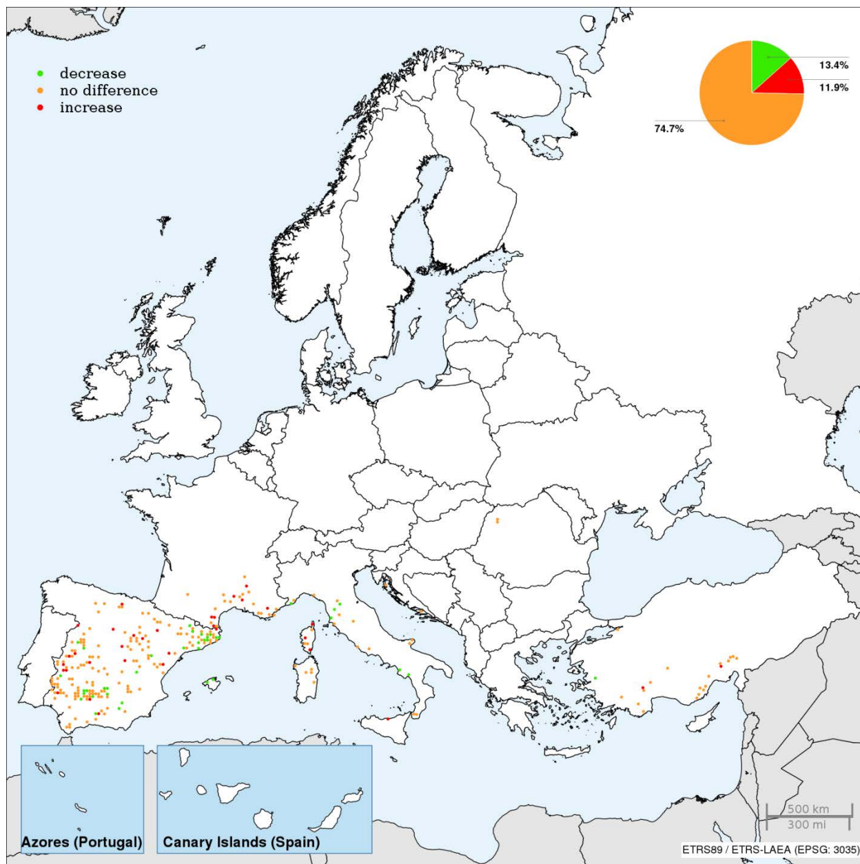
Annex I-9. Trends of mean plot defoliation (Mann-Kendall test) of evergreen oaks ( Quercus coccifera , Q. ilex , Q. rotundifolia , Q. suber ) between 2006 and 2014 with a minimum assessment length of 5 years.
