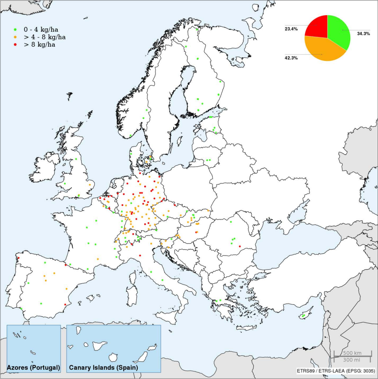
Figure 6-4. Throughfall (and stemflow where applicable) deposition of ammonium nitrogen ( \text{NH}_4\text{-N} ) in European forests in 2013.
