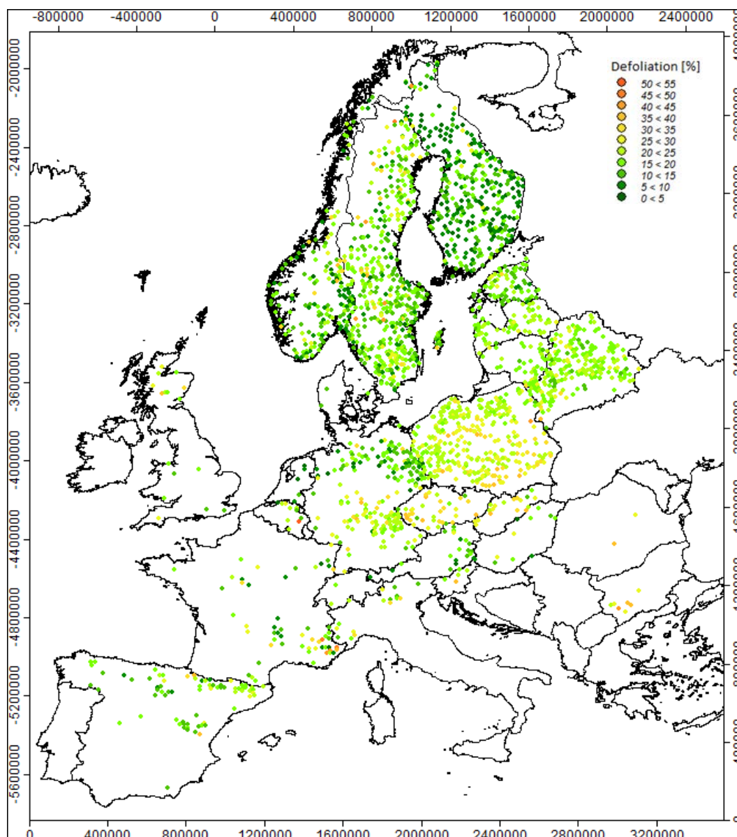
Figure 4-1. Plot-related defoliation estimates for Scots pine ( Pinus sylvestris ): medium-term means from 1999 to 2005.
